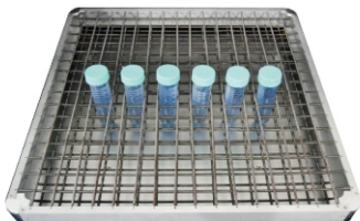
Platform SPW-420 W.410 x D.420 x H.65mm
